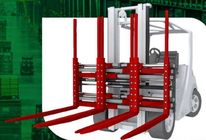
TRIPLE PALLET HANDLER ON A PANTOGRAPH T429/T149Z
